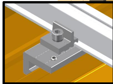
Integration with Railed system connection on horizontal rib
