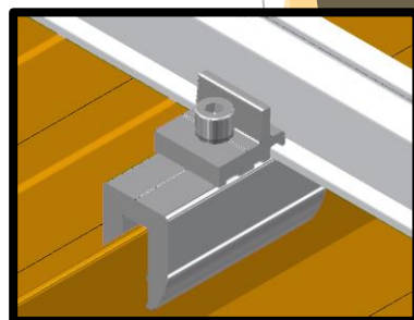
Integration with Railed system connection on standing rib
