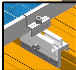
Integration with PV module connection
